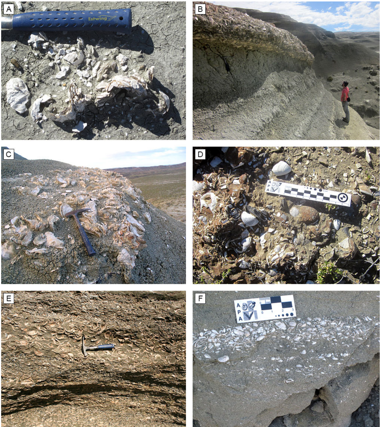
Figure 4. Field photographs of fossil concentrations of the MOM. a-c) Biogenic concentrations. a) Isolated clumps of Crassostrea orbignyi at Cañadón de La Chacra, formed by mostly white small and thin shelled specimens embedded in fine-grained silty tuffaceous sandstone matrix. b) View of one of the C. orbignyi reefs at Cerro Observación. c) Close-up views of one C. orbignyi reefs at Cerro Observación, including mostly white thin shelled specimens embedded in silstone matrix. d-e) Sedimentologic concentrations. d) Polytypic sedimentologic concentration at Cerro Monte León showing densely-packed and bimodal fabric, formed by highly abraded valves of C. orbignyi and valves and fragments of other mollusks in chaotic orientation. e) Monotypic sedimentologic concentration at Cerro Redondo locality, composed of fragments, valves and articulated specimens of C. orbignyi mostly concordant to bedding, inside of cross-stratified coarse-grained to conglomeratic sandstone. f) Mixed biogenic-sedimentologic concentration at Cañadón de La Chacra, composed mostly of specimens of Maclridae parallel to the stratification and convex-up oriented. Hammer handle for scale ~28 cm.
