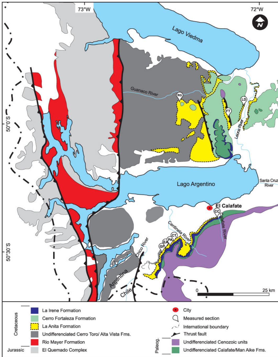
Figure 3. Geological map of the study area showing the distribution of stratigraphic units of the Austral-Magallanes Basin (modified from Kraemer and Riccardi, 1997; Ghiglione et al. , 2014). Measured section names: RG = Río Guanaco; FT = Filo del Turbio; LD = Luz Divina; GF = Galpón de Freile; EA = Estancia Anita; PA = Paredón; CT = Campo Tropilla; and CC = Cerro Calafate.
