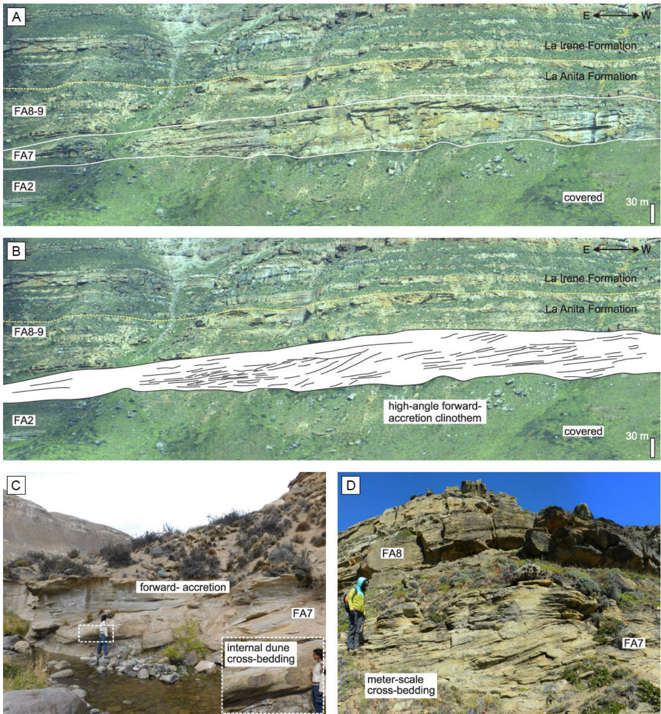
Figure 11. Representative outcrop photographs of Facies Association 7. a) and b) Outcrop panels showing high-angle forward-accretion clinothem dipping toward the southeast. c) Detail of the forward-accretion clinothem. The inset in Fig. 11c shows detail of internal dune cross-bedding dipping in the same direction as the clinothem. d) Detail of internal large-scale dune cross-bedding.
