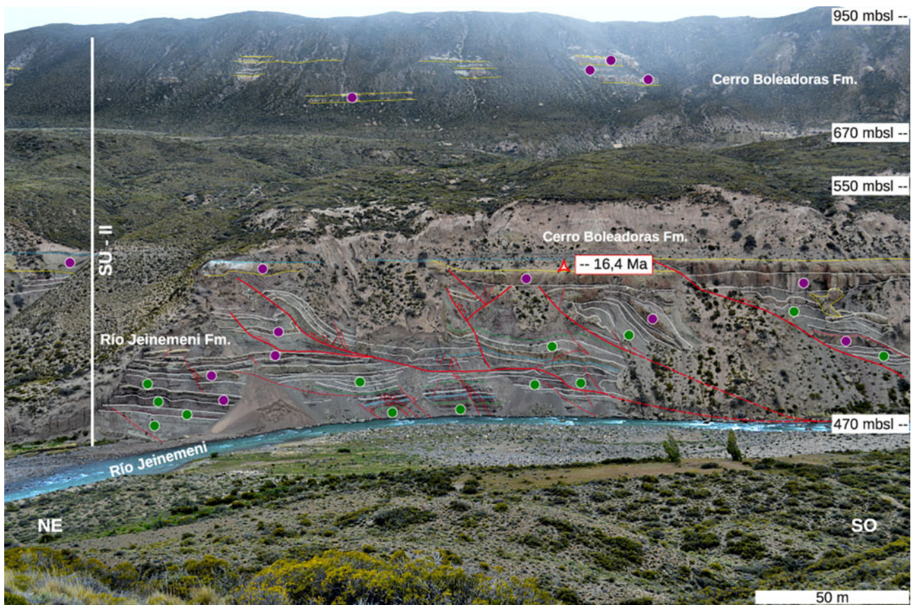
Figure 14. Photographic panoramas looking to the NW of Río Jeinemeni exposures showing superposition of extensional and compressional deformational structures during deposition of the Río Jeinemeni Formation (lower Miocene) (modified from Barberón et al. , 2018). The red star represents an U-Pb age from Folguera et al. , 2018. Green and purple dots represent FA III and FA IV, respectively. These deposits are associated in Sedimentary Unit II, a mixed-load fluvial system. The subhorizontal, post-deformation strata belong to the Cerro Boleadoras Formation.
