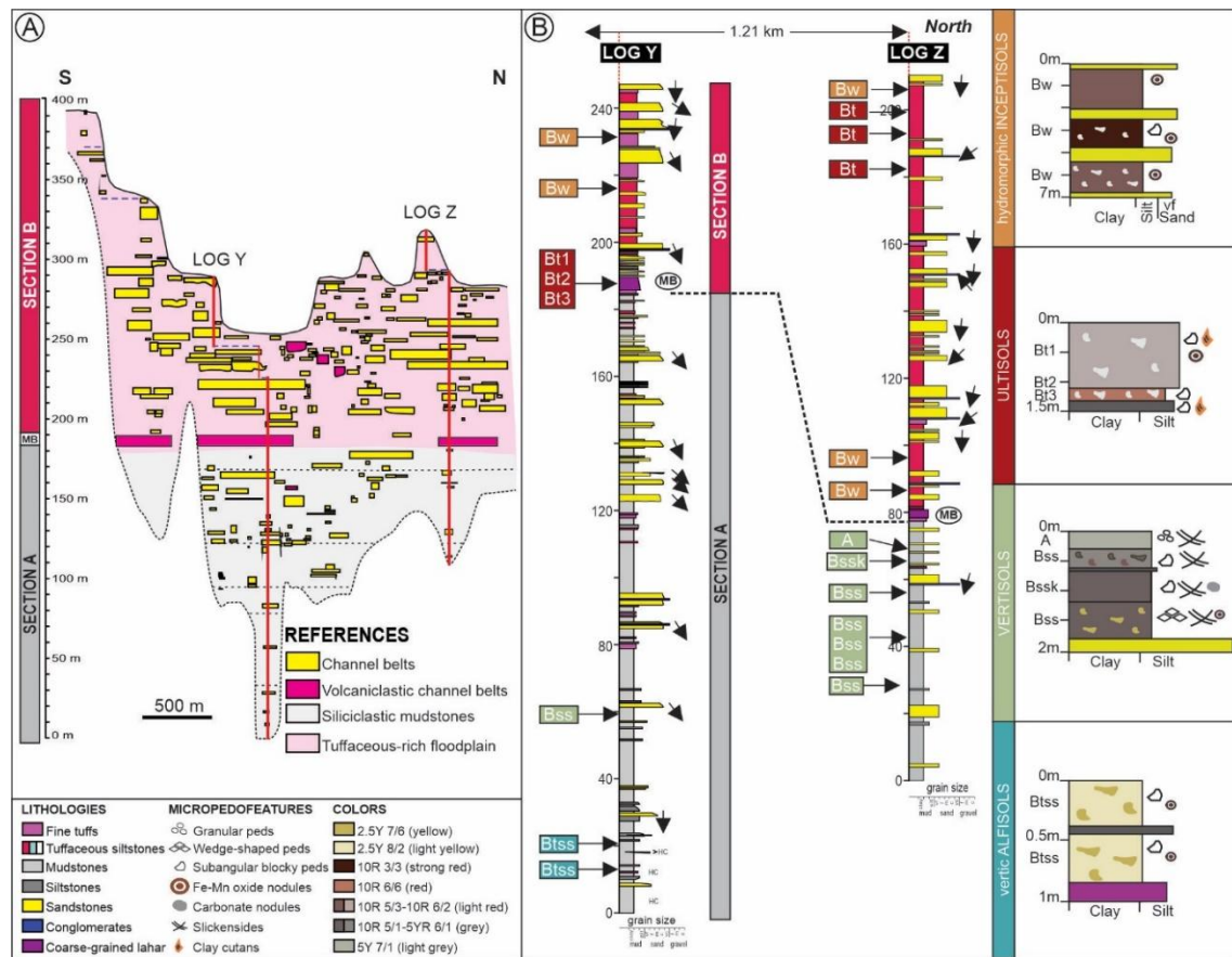
Figure 5. The Bajo Barreal Formation in the Cerro Ballena anticline. a) Macro-architecture of the unit and location of sedimentological profiles (after Paredes et al. , 2018b). b) Sedimentological and paleopedological sections were measured from the Bajo Barreal Formation in the Cerro Ballena (logs Y and Z). The four pedotypes were represented in stratigraphic order of appearance with a representative profile (for details see Lizzoli et al. , 2025).
