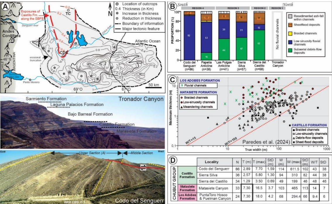
Figure 3. The Castillo-Mina del Carmen depositional system. a) Thickness distribution in the GSJB (after Fitzgerald et al. , 1990). Pictures show typical aspects of the unit at the northern basin margin (Tronador Canyon) and in the Codo del Senguerr anticline. b) Spatial variation of the channel types of the Castillo Formation along the SBF, from exposures of the northern basin margin to the exposures at the Codo del Senguerr anticline. c) A scatter log-log plot shows the relationship between maximum thickness and true width (calculated normal to the mean paleoflow direction) of channel deposits of the Los Adobes, Matasiete, and Castillo formations. d) Geometrical parameters of fluvial channel belt deposits of the Los Adobes, Matasiete, and Castillo formations in the SBF.
