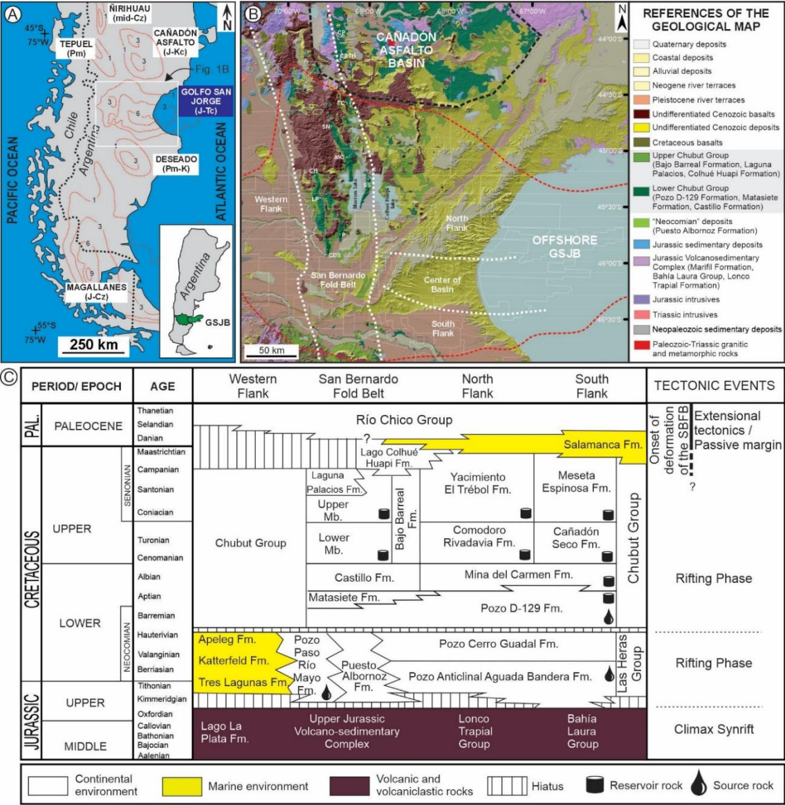
Figure 1. a) Location and thickness map (in Km) of sedimentary basins in central Patagonia, Argentina (after Paredes, 2023). The inset shows the extent of the Golfo San Jorge Basin in green. b) Geological map of the Golfo San Jorge Basin, main structural subdivisions and localities mentioned in the text. CP: Cañadón Puelman, CPTH: Cerro Punta Toro Hosco, TC: Tronador Canyon, SN: Sierra Nevada anticline, MC: Matasiete Canyon, SS: Sierra Silva anticline, LP: Las Pulgas anticline, P: Papelía anticline, CDS: Codo del Senguerr anticline, CB: Cerro Ballena anticline. c) Mesozoic to Paleogene stratigraphy.
