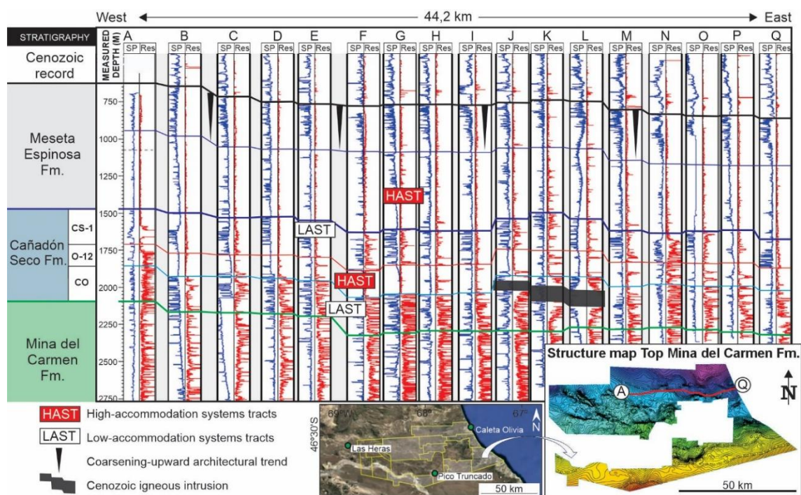
Figure 4. Well-log correlations of the Cañadón Seco and Meseta Espinosa formations, South Flank of the GSJB. Vertical changes in the stacking density of the Cañadón Seco Formation: the Caleta Olivia (CO) and the CS-1 members comprise low-accommodation systems tracts, whereas the O-12 Member represents a high-accommodation systems tracts, dominated by
